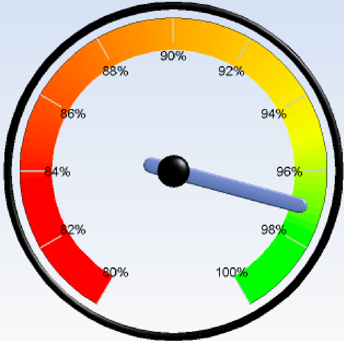
Percent Attendance
